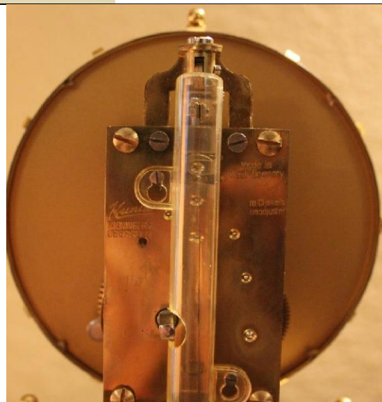
WNS-CLK-133 - Kundo - Oval 400 day clock - Movement Markings View
